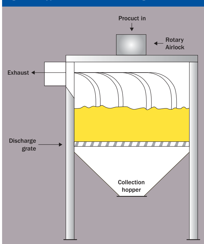
Figure 2 - Typical vertical cooler arrangement
