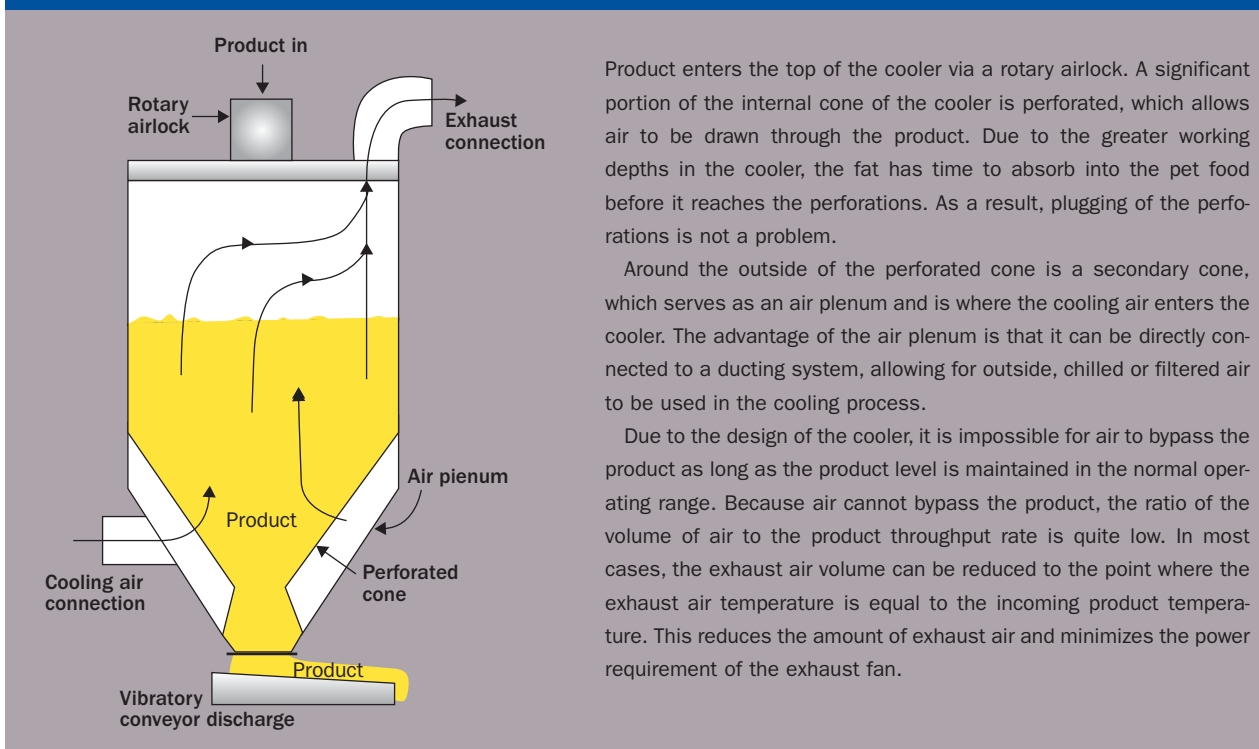
Figure 3 - Illustration of a vertical cooler manufactured by Extru-Tech
